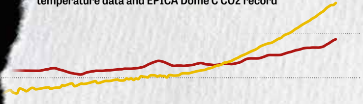
Original References: Greenland GISP2 Ice Core temperature data and EPICA Dome C CO2 record
